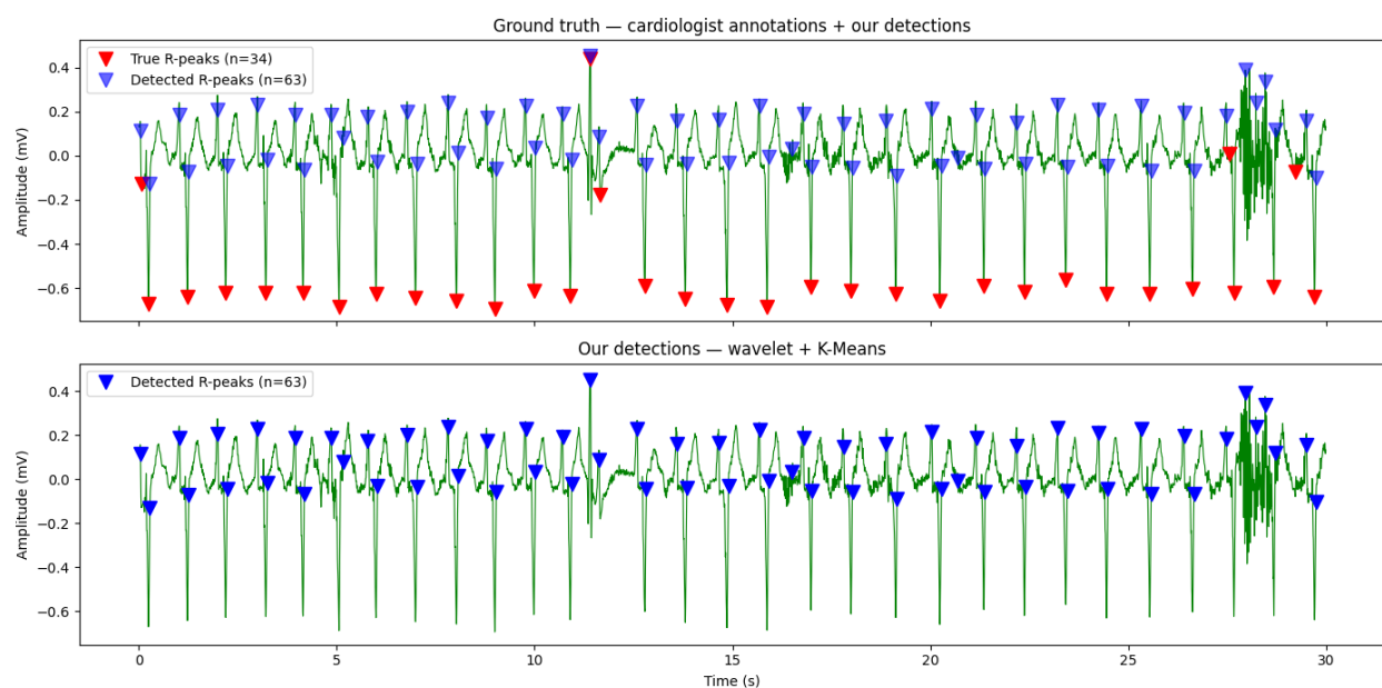
Figure 14: R-peak detections for Record 108 before polarity correction.
