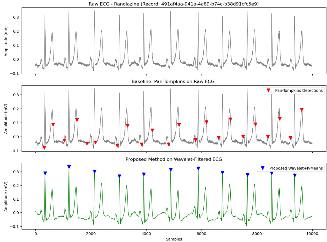
Figure 19: Pan-Tompkins vs. Proposed Method.
