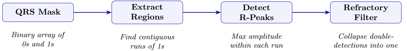
Figure 10: The three sequential sub-steps of R-peak extraction.
